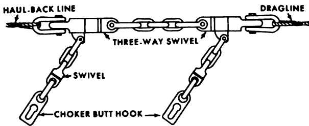
Figure 7-12. Two types of butt rigging for a high-lead system.
